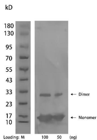
Figure 1. Detection of streptavidin fusion protein were analyzed by Western blot using Rabbit Anti Streptavidin Antibody, pAb (Cat.DTA0231 , at 1 \mu\text{g/mL} concentration).
